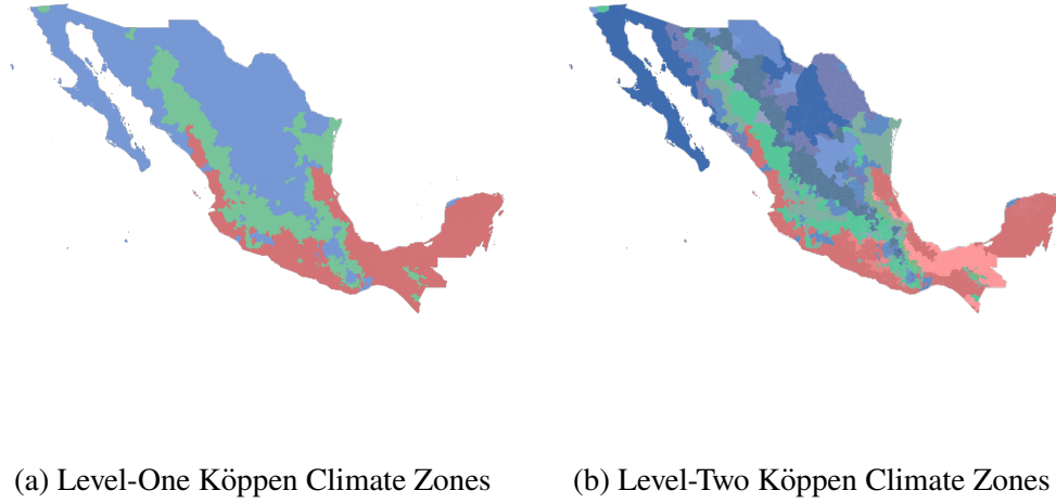
Figure 4: Köppen Climates in Mexico
