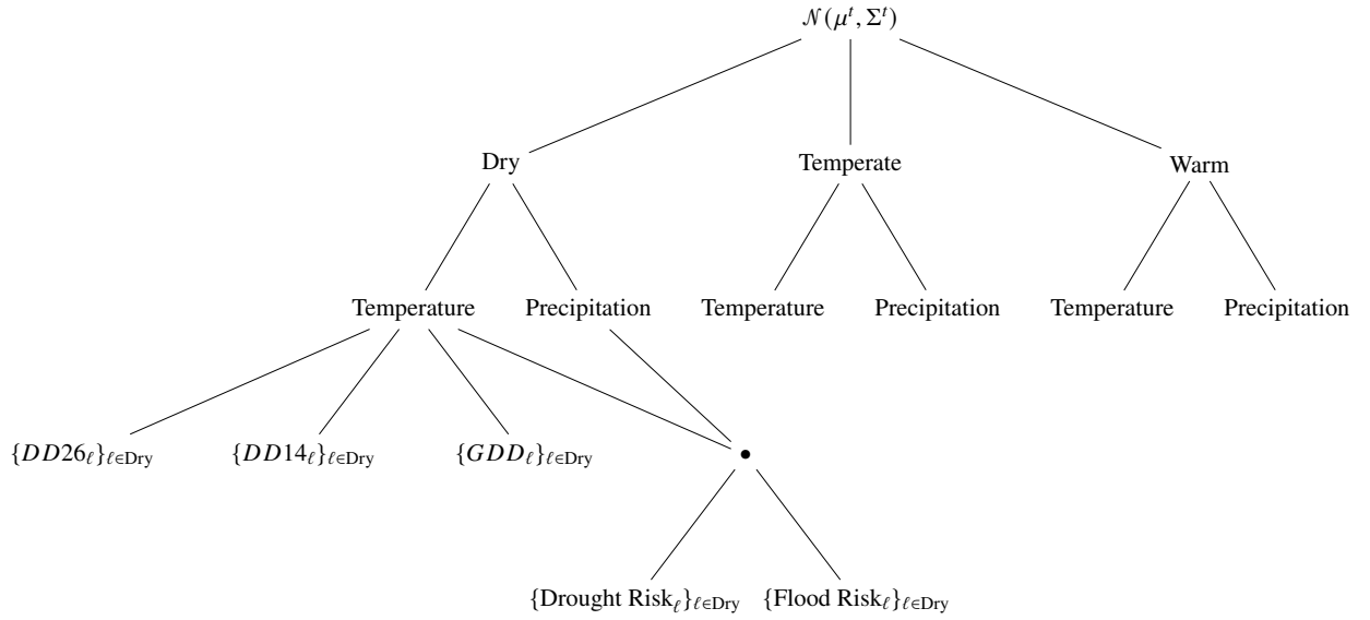
Figure 5: Graphical Representation of the Climate Model
